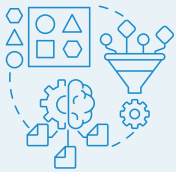
Machine Learning
